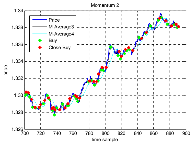
Fig. 5c Sample performance of Momentum 2 strategy
