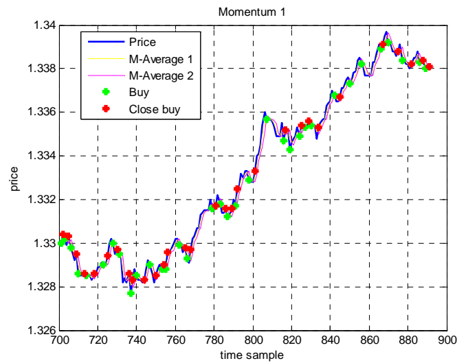
Fig. 5b Sample performance of the Momentum 1 strategy
